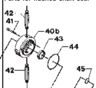
Parts for flushed shaft seal
