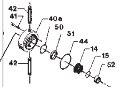
Parts for double mechanical shaft seal
