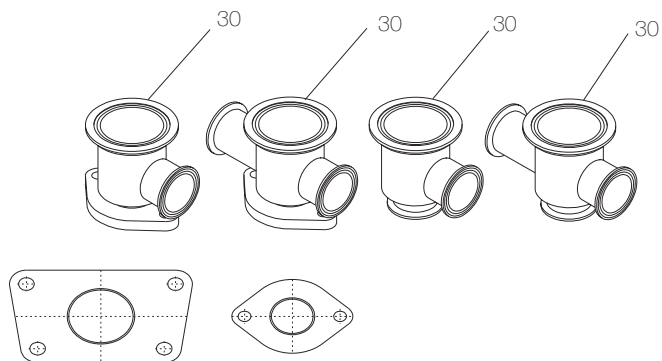
4 hole flange for 2½" and 3" valves
