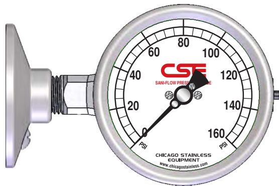
2-1/2" LEFT SIDE MOUNT (Shown with 1-1/2" Tri-Clamp)
