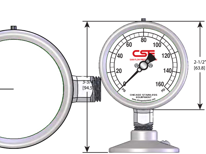
2-1/2" BOTTOM MOUNT (Shown with 1-1/2" Tri-Clamp)
