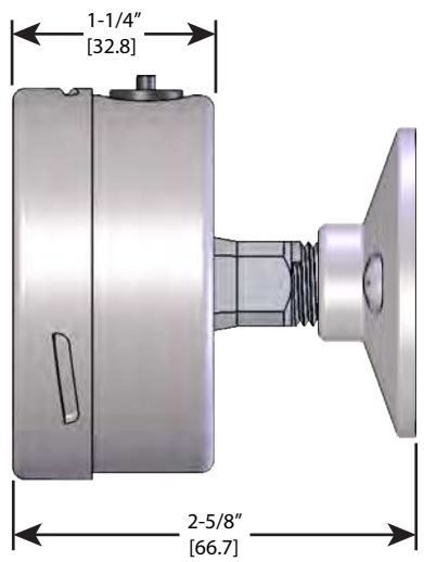
2-1/2" BACK MOUNT (Shown with 1-1/2" Tri-Clamp)
