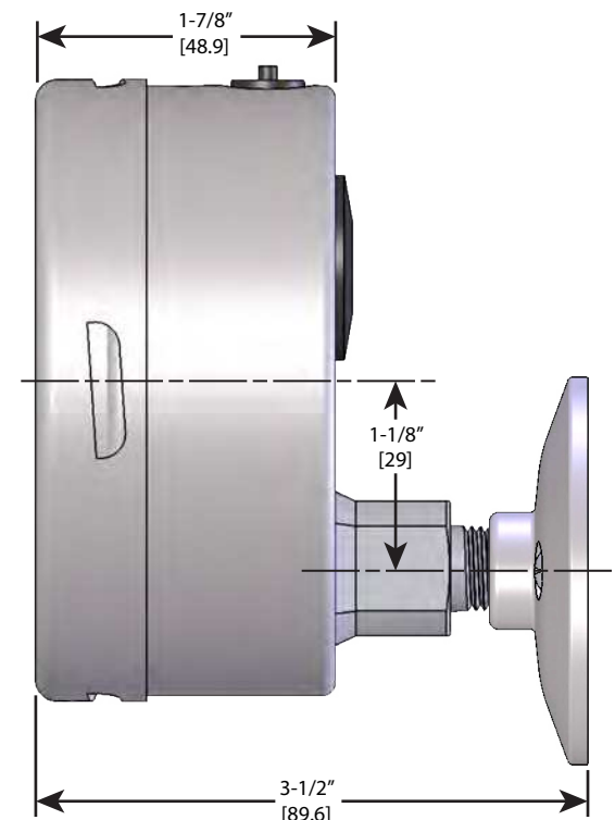
4" BACK MOUNT (Shown with 2" Tri-Clamp)
