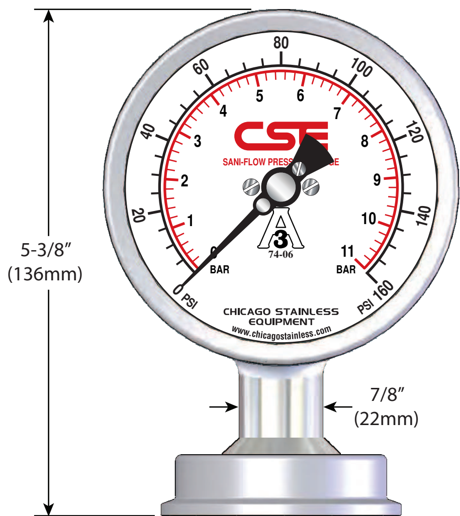
3-1/2" BOTTOM MOUNT (Shown with 2" Tri-Clamp)
