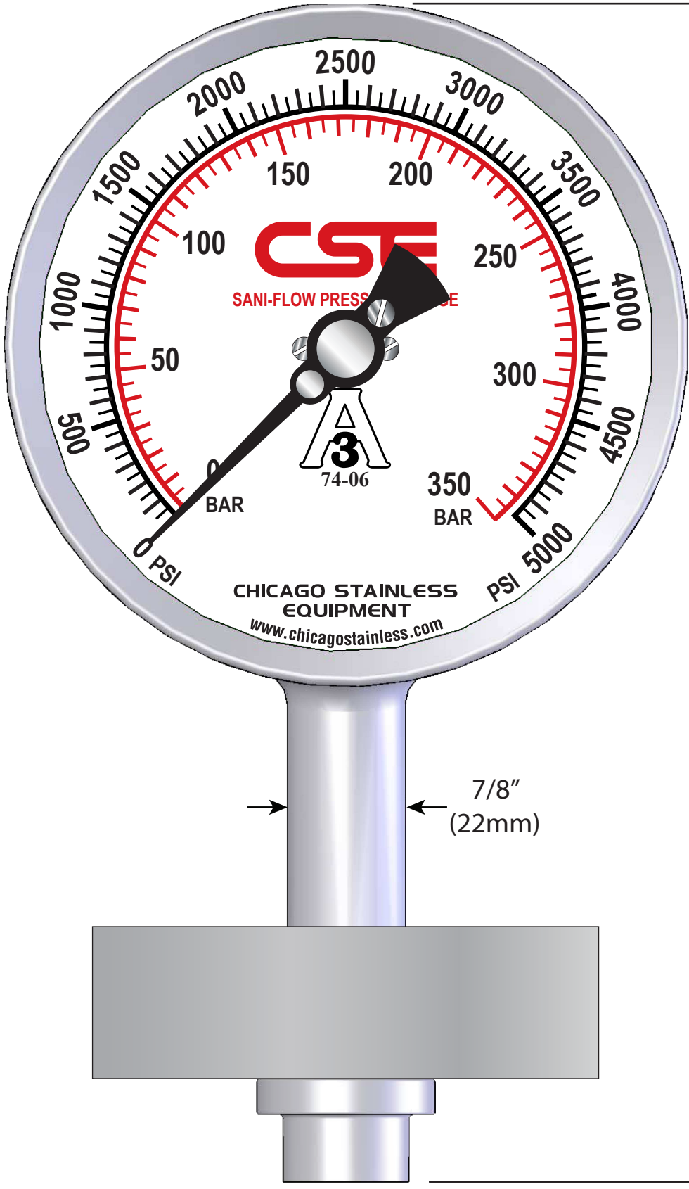
FRONT VIEW (Shown with 2 Bolt Flange)
