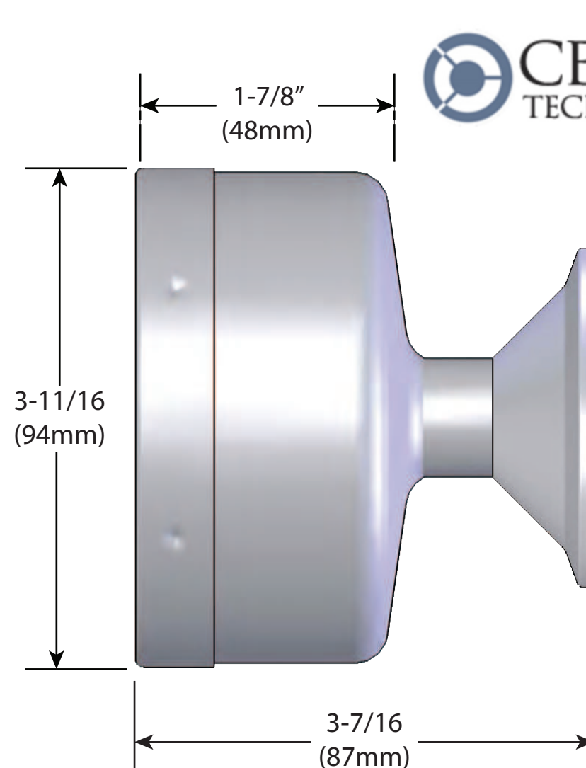
3-1/2" BACK MOUNT (Shown with 2" Tri-Clamp)
