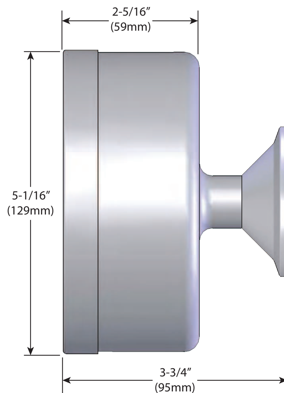
5" BACK MOUNT (Shown with 2" Tri-Clamp)
