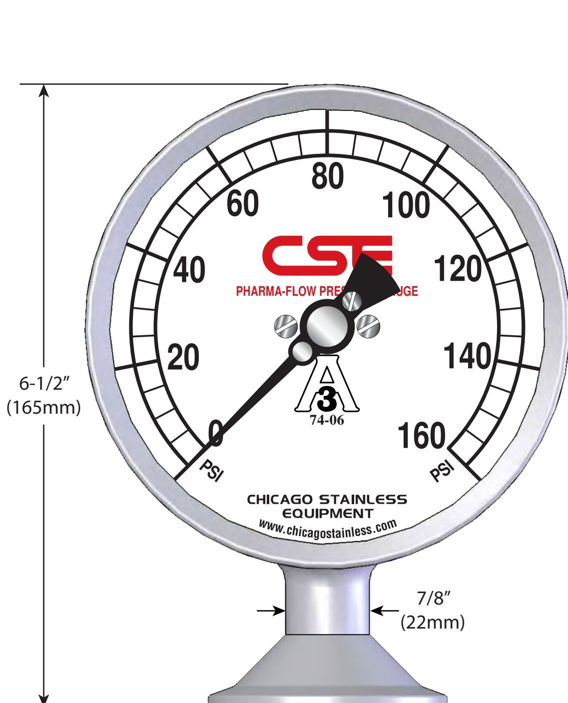
5" BOTTOM MOUNT (Shown with 2" Tri-Clamp)
