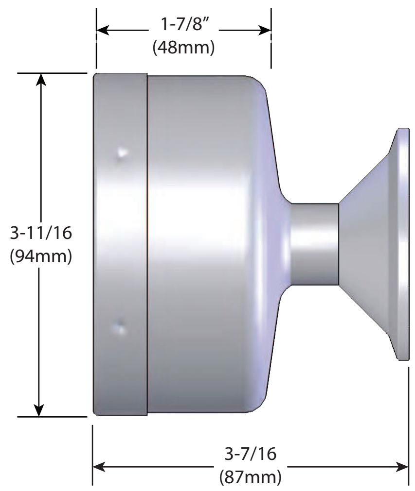
3-1/2" BACK MOUNT (Shown with 2" Tri-Clamp)
