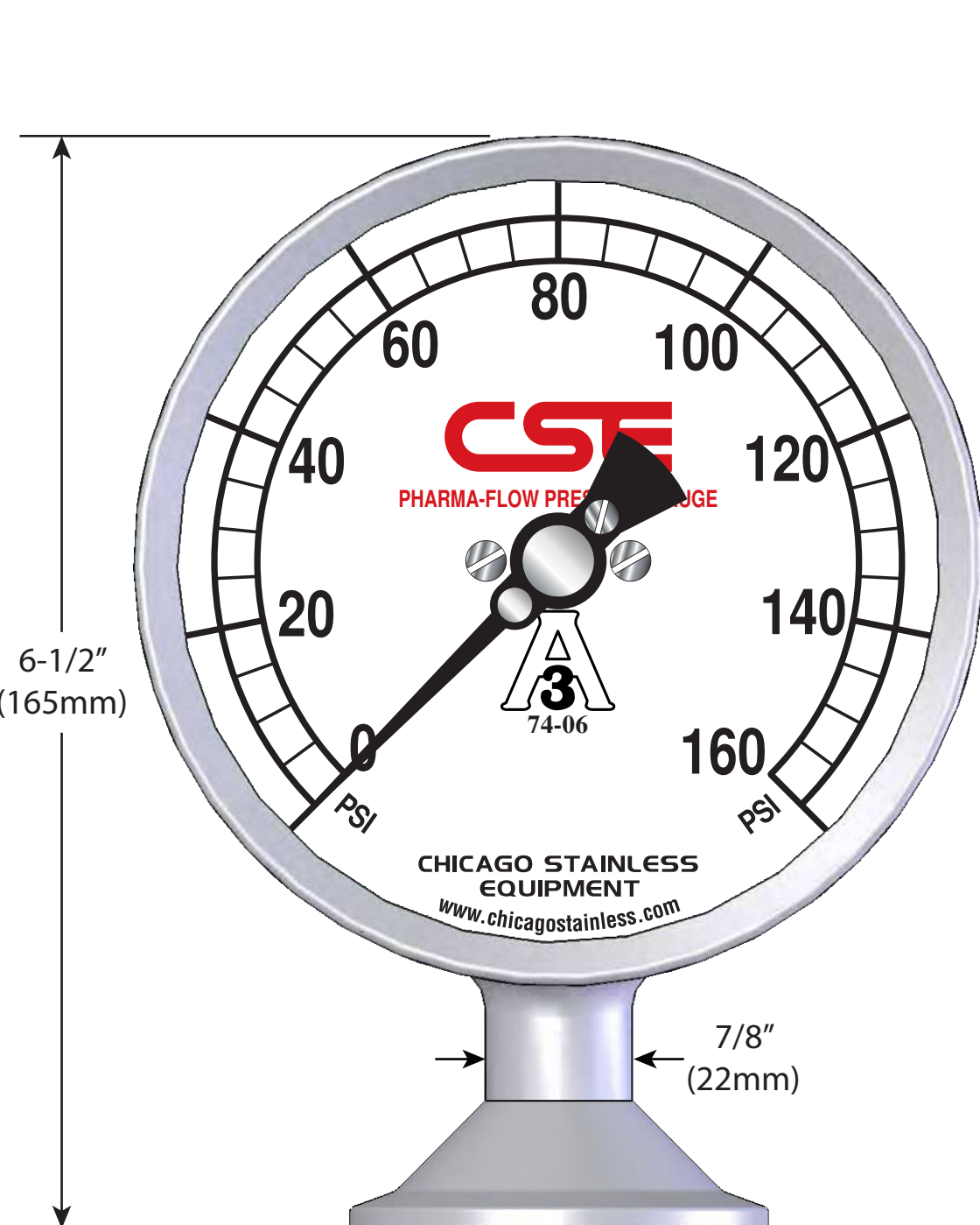
5" BOTTOM MOUNT (Shown with 2" Tri-Clamp)
