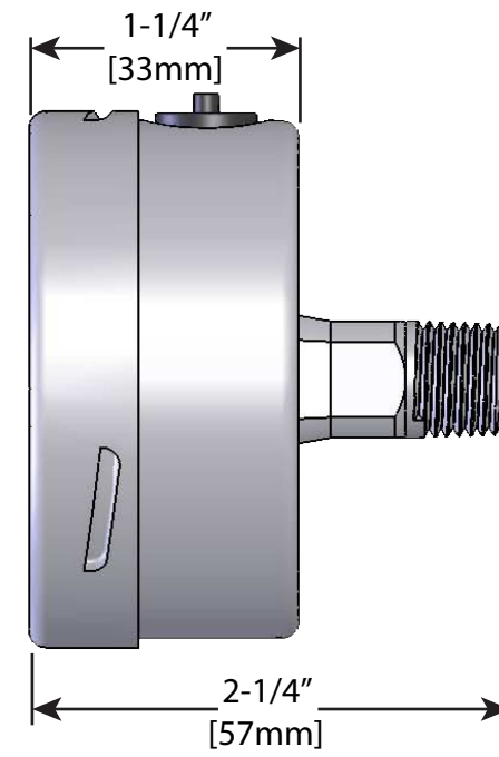
2-1/2" BACK MOUNT
