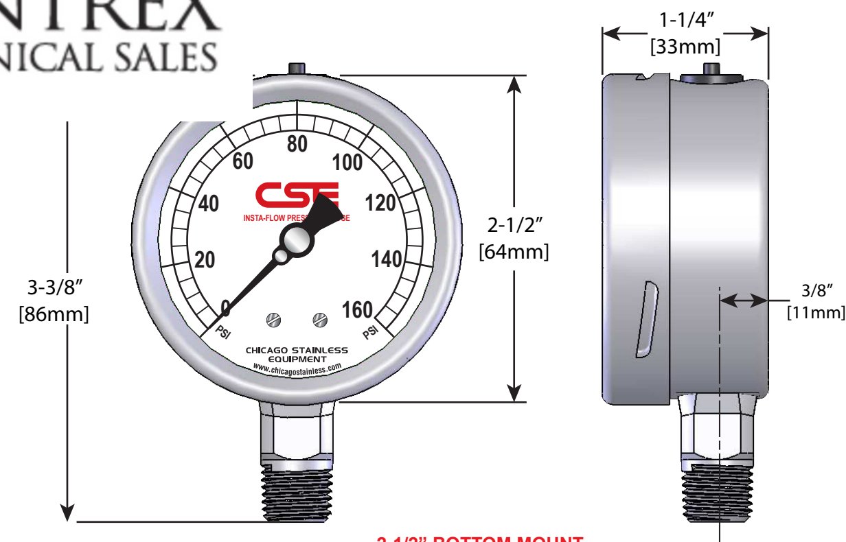
2-1/2" BOTTOM MOUNT
